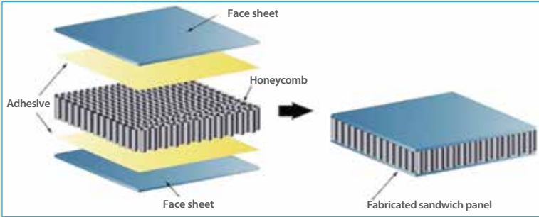
Figure 5: Schematic view of a composite sandwich panel.
