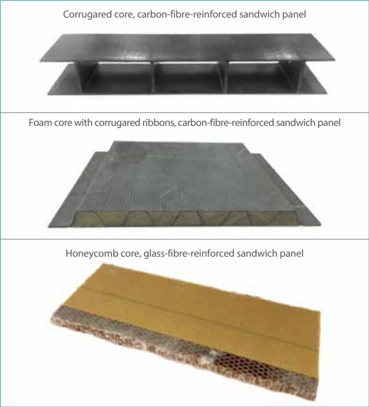
Figure 4: Different types of composite sandwich panels
