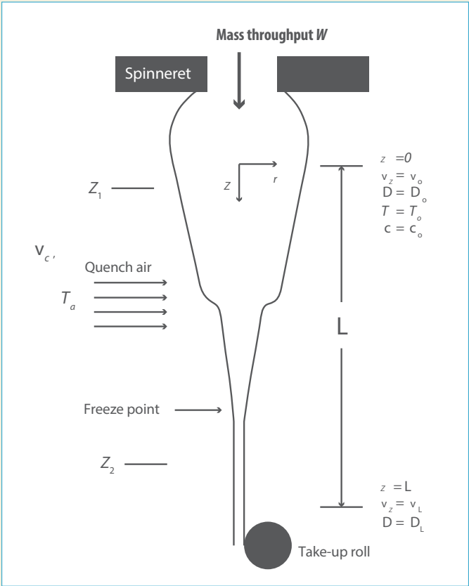
Figure 1: Melt Spinning
